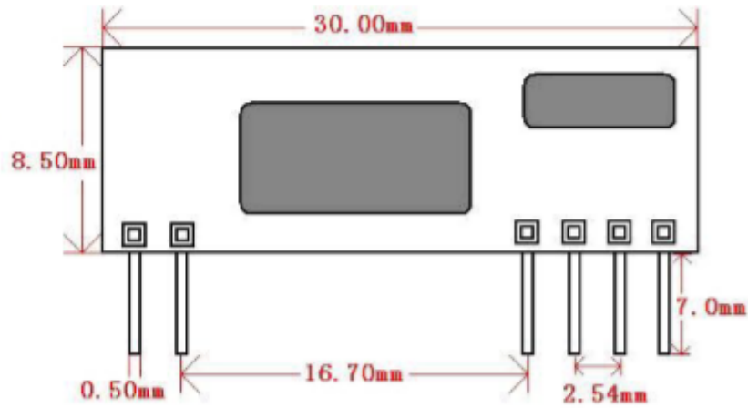
Figure2 CY48 Dimension
